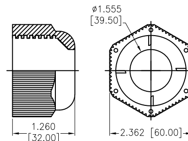
Sealing Nut
