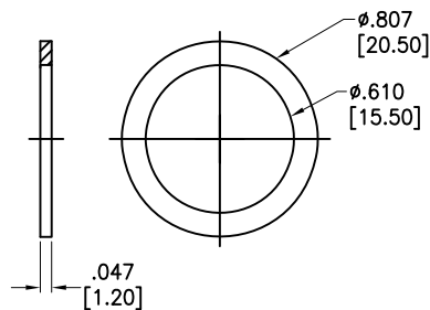
Ⓑ Washer
