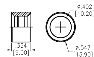
Ⓓ Seal
