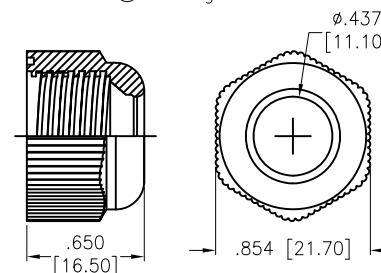
Ⓔ Sealing Nut
