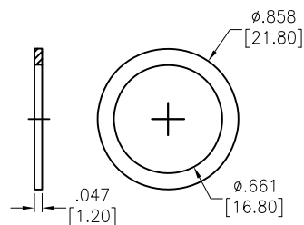
Ⓑ Washer
