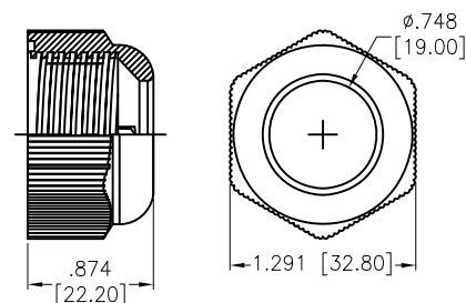
Ⓔ Sealing Nut
