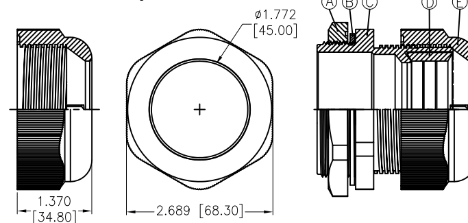
Ⓔ Sealing Nut
