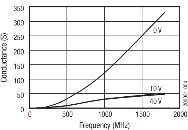
Figure 4. Conductance vs Frequency and Reverse Voltage
