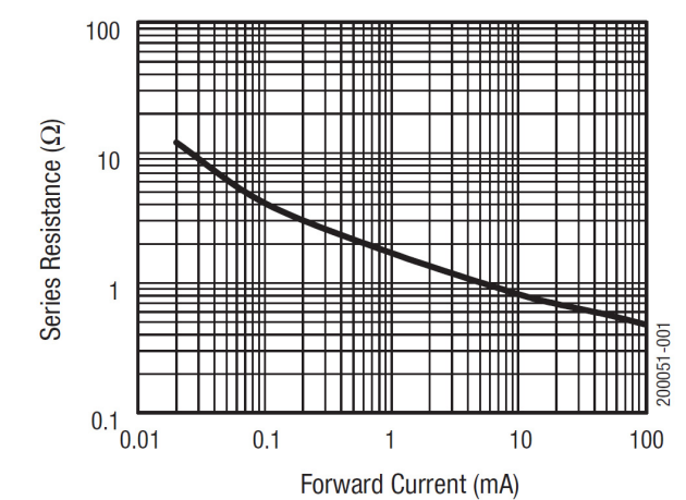
Figure 1. Series Resistance vs Current @ 100 MHz
