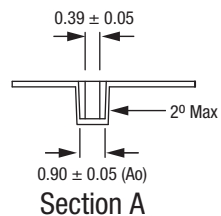
Figure 6. SC-79 Tape and Reel Dimensions
