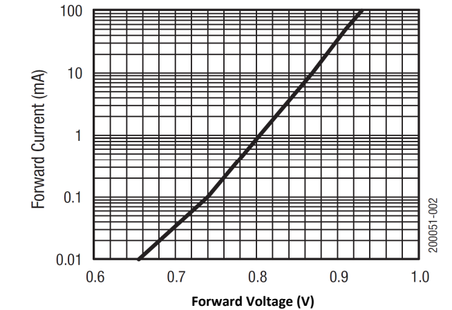
Figure 2. Forward Current vs Voltage
