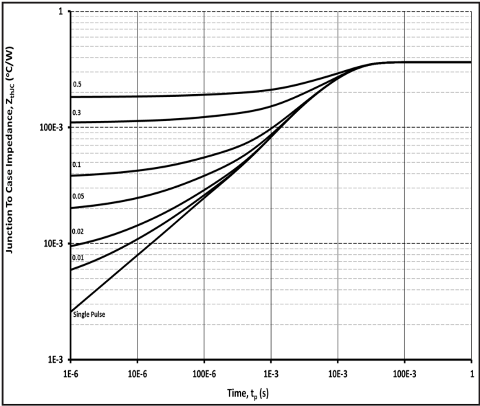
Figure 8. Transiant Thermal Impedence
