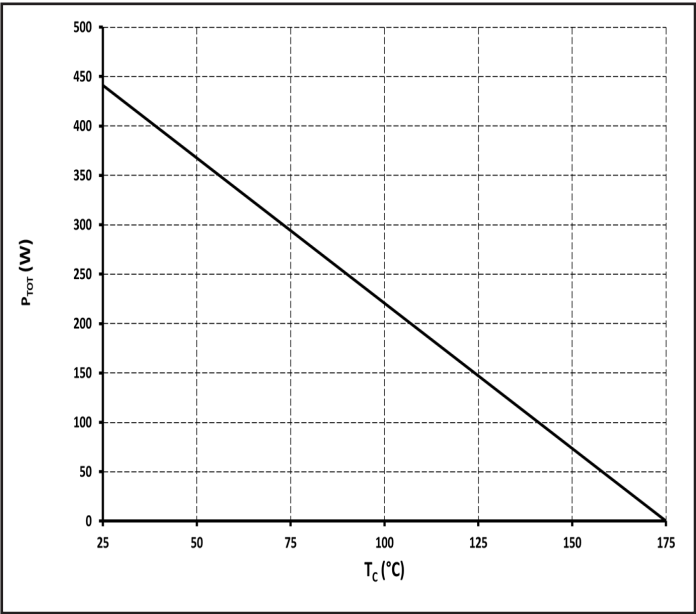
Figure 4. Power Derating
