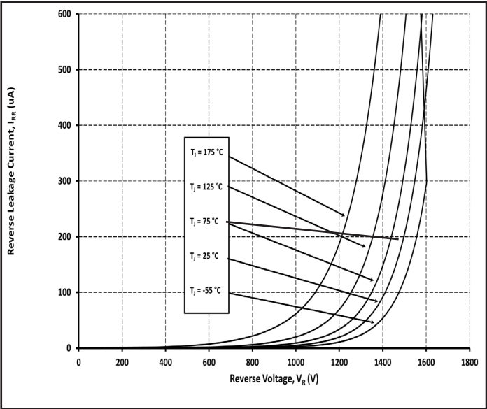
Figure 2. Reverse Characteristics
