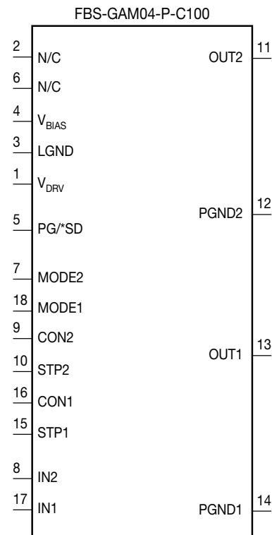
Figure 14. Suggested BS-GAM04-P-C100 Schematic Symbol
