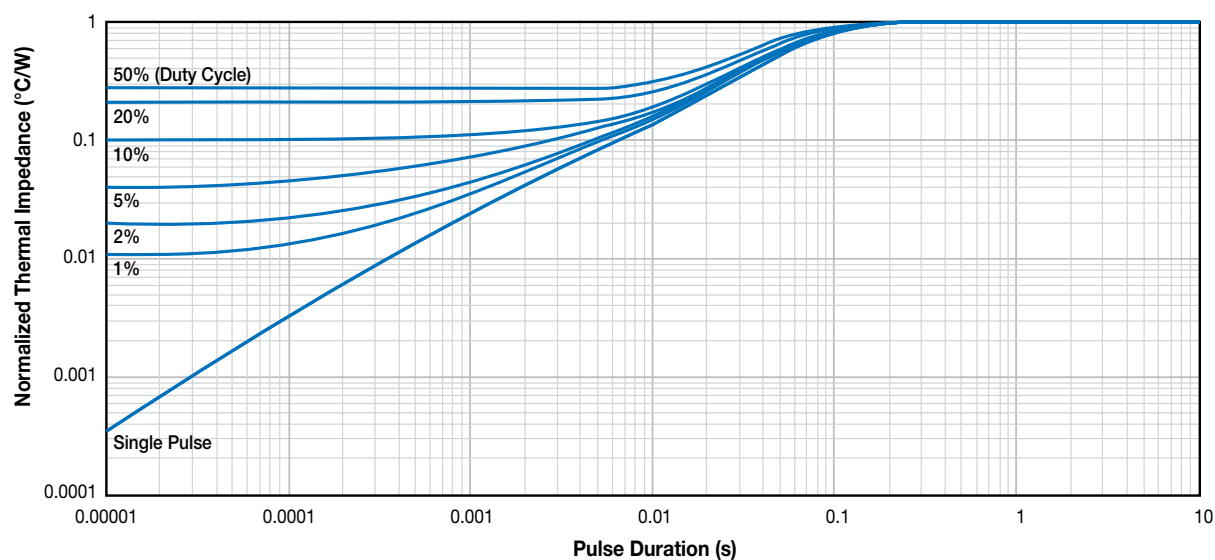
Figure 15. Typical Power eGAN ® HEMT Normalized Junction-to-Case Thermal Impedance
