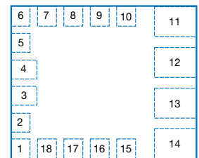
Bottom (Pad) View
