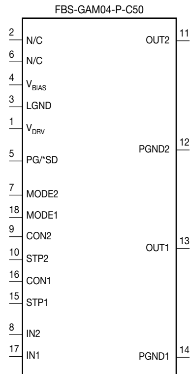
Figure 14. Suggested FBS-GAM04-P-C50 Schematic Symbol
