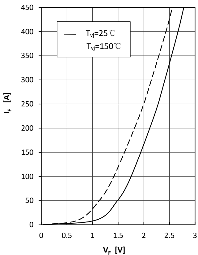
Fig7.Diode Foward Characteristics
