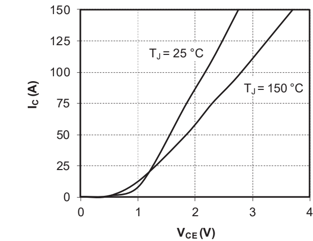
Figure 1-17. Output Characteristics (V GE = 15V)
