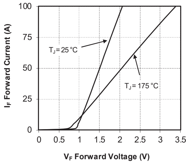
Figure 1-9. Forward Characteristics
