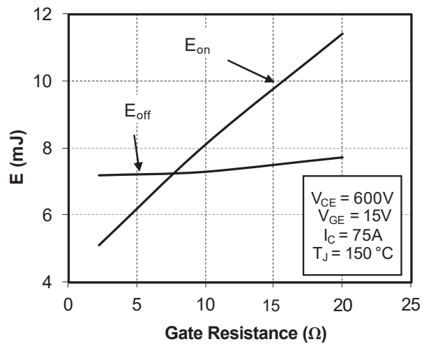
Figure 1-21. Switching Energy Losses vs. Gate Resistance
