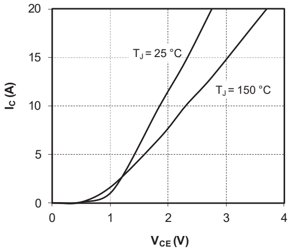
Figure 1-12. Output Characteristics ( V_{GE} = 15\text{V} )
