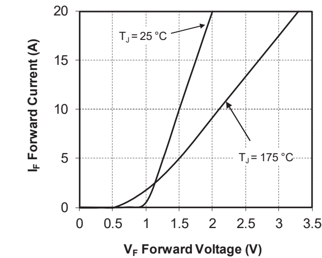
Figure 1-14. Forward Characteristics
