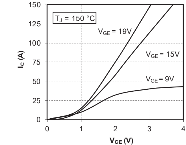
Figure 1-18. Output Characteristics
