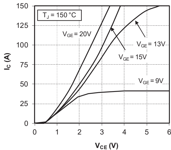
Figure 1-3. Output Characteristics, T_J = 150^{\circ}\text{C}
