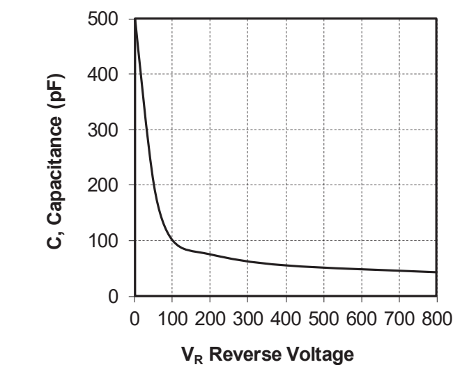
Figure 1-15. Capacitance vs. Reverse Voltage
