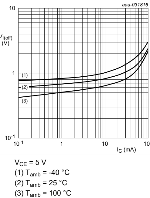
Fig. 7. NHDTC123JU: Off-state input voltage as a function of collector current; typical values
