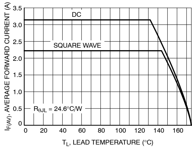
Figure 6. Current Derating
