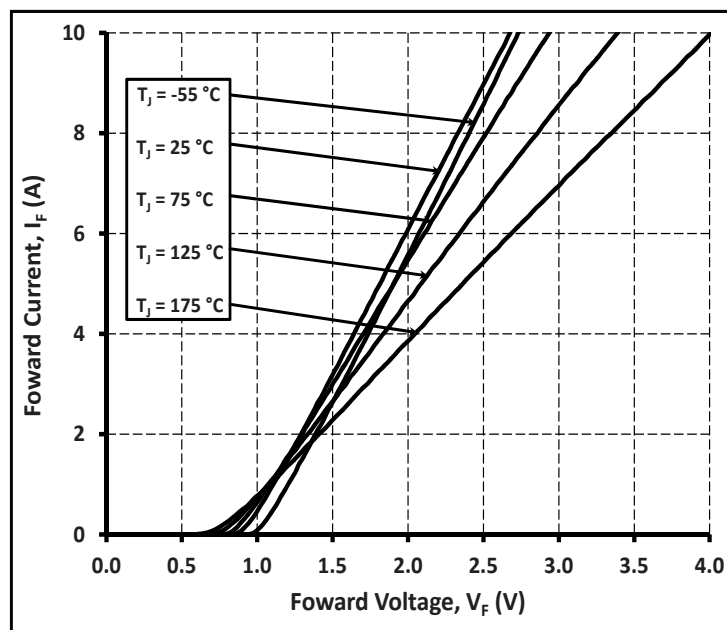
Figure 1 Forward Characteristics
