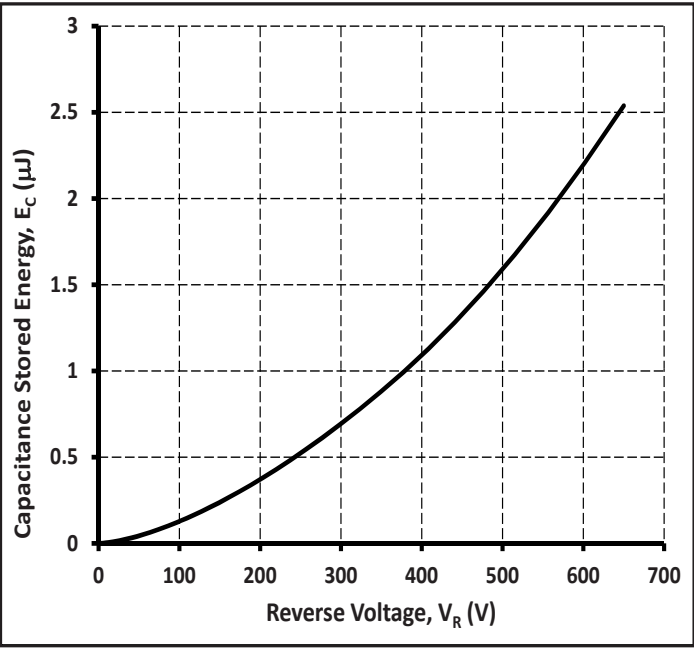
Figure 7 Capacitance Stored Energy
