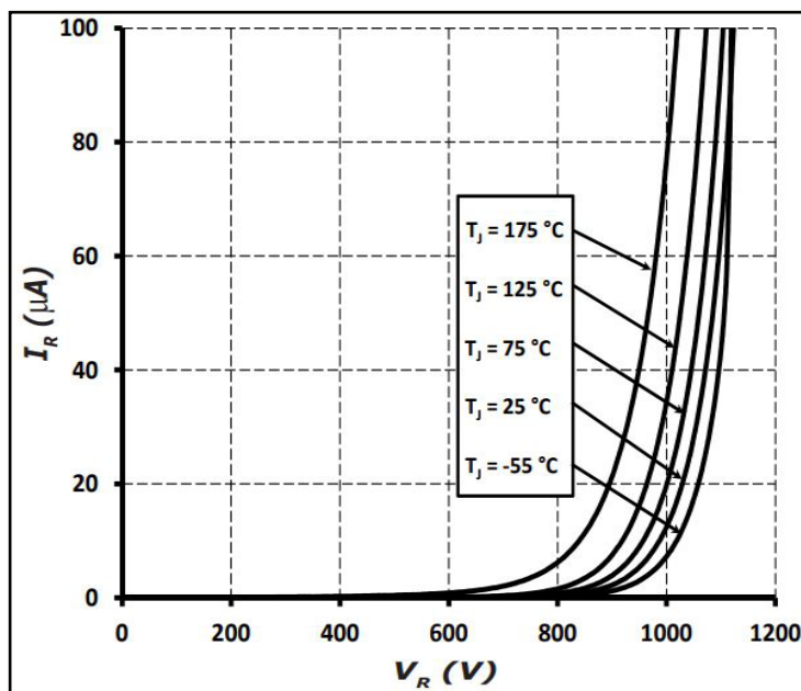
Figure 2 Reverse Characteristics
