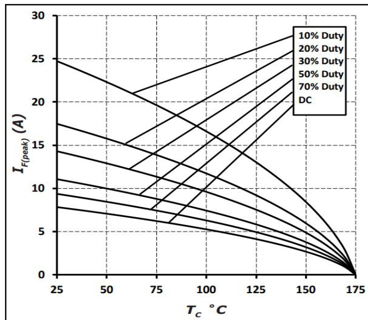
Figure 3 Current Derating
