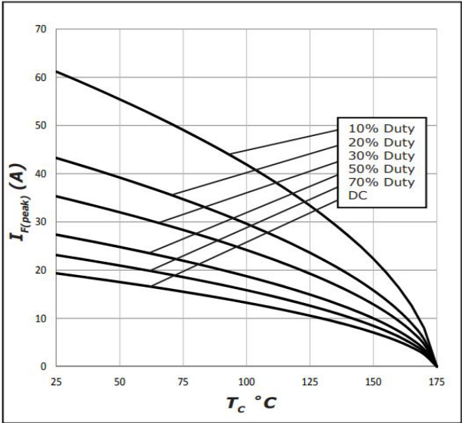
Figure 3 Current Derating
