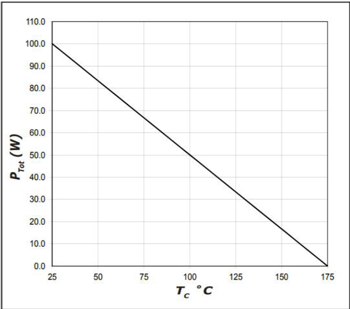
Figure 4 Power Derating
