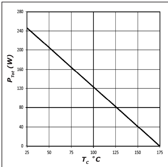
Figure 4. Power Derating
