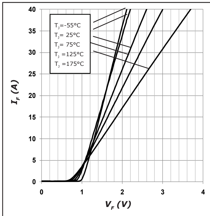
Figure 1. Forward Characteristics
