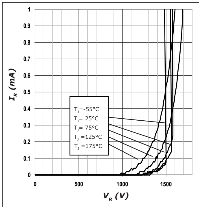
Figure 2. Reverse Characteristics
