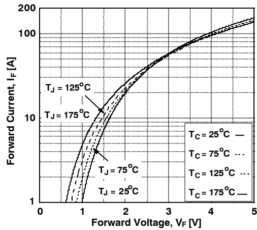
Figure 19. Forward Characteristics
