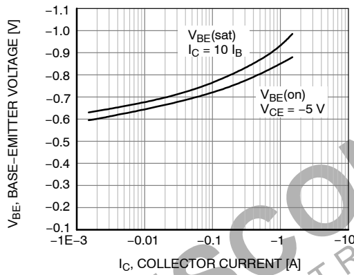
Figure 3. Base-Emitter Voltage
