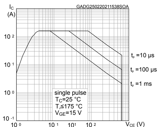
Figure 12. Forward bias safe operating area for TO-3PF
