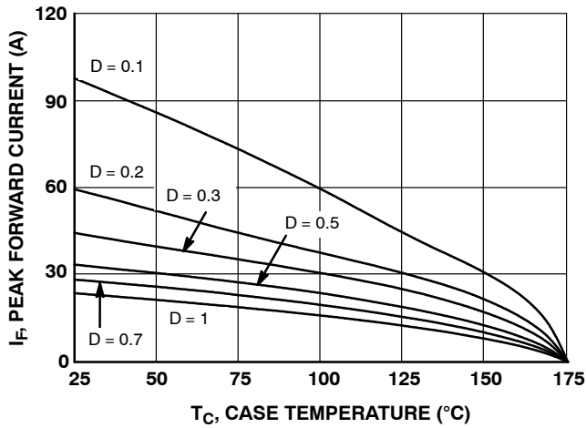
Figure 3. Current Derating
