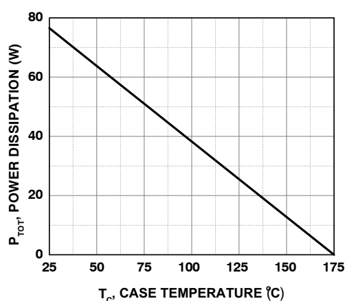
Figure 4. Power Derating
