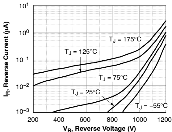
Figure 2. Reverse Characteristics
