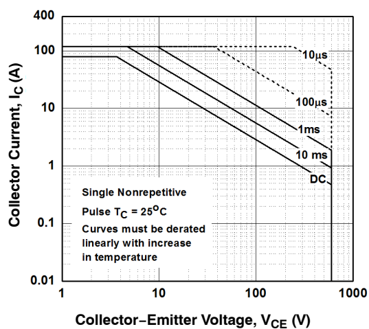
Figure 11. SOA Characteristics
