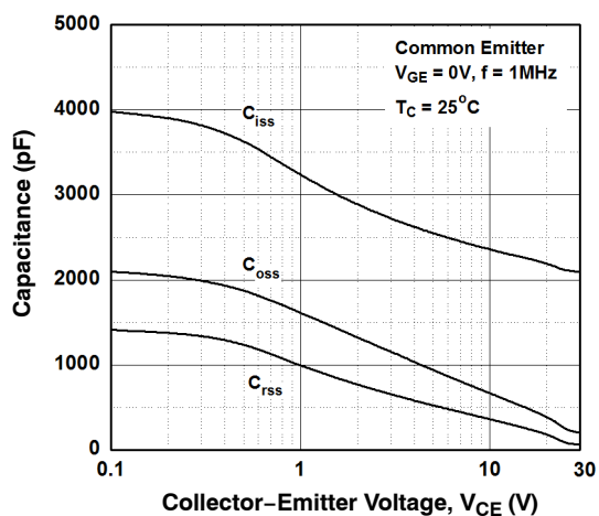
Figure 9. Capacitance Characteristics
