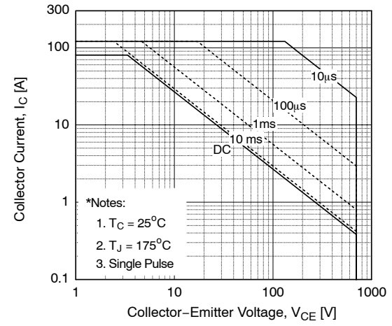
Figure 16. SOA Characteristics
