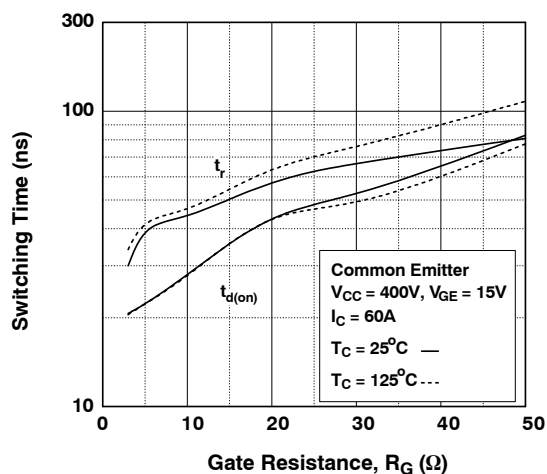
Figure 13. Turn-on Characteristics vs. Gate Resistance
