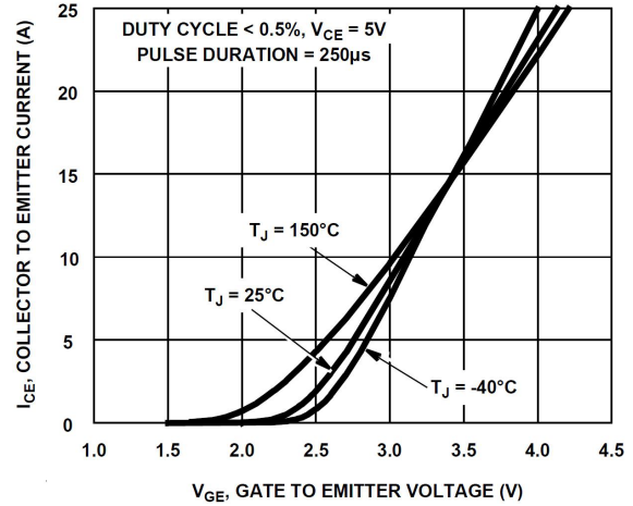
Figure 8. Transfer Characteristics
