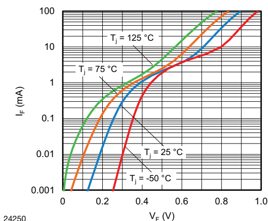
Fig. 3 - Typical Forward Current vs. Forward Voltage
