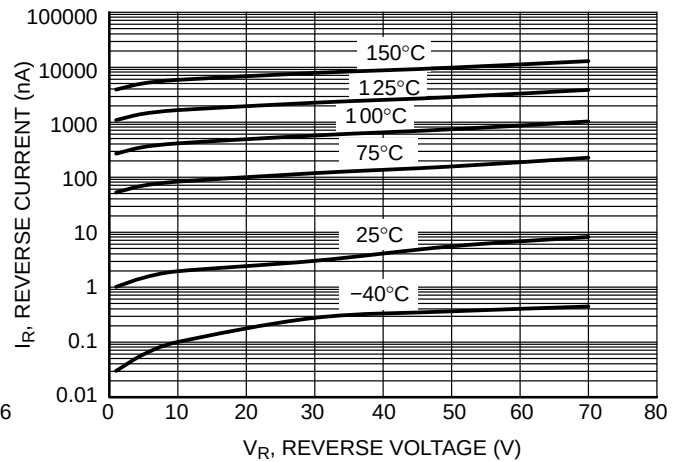
Figure 2. Reverse Current versus Reverse Voltage
