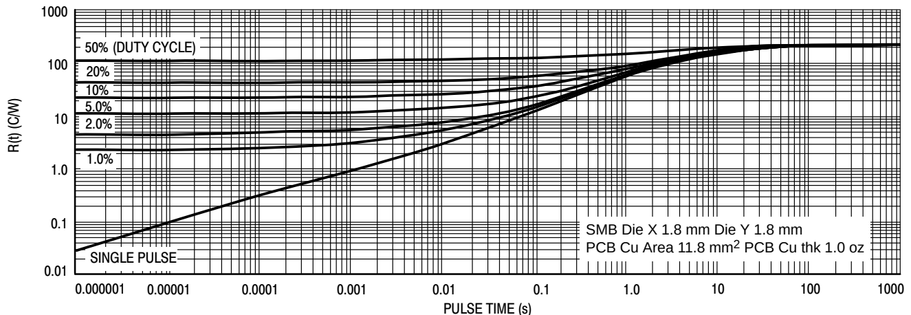
Figure 10. Thermal Response, Junction-to-Ambient (min pad) – MBRS2H100T3G/NBRS2H100T3G/NBRS2H100NT3G
