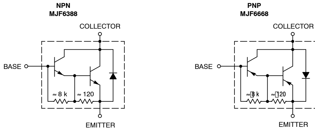
Figure 1. Darlington Schematic
