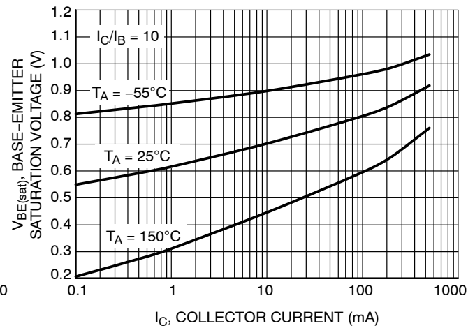
Figure 7. Base Emitter Saturation Voltage vs. Collector Current
