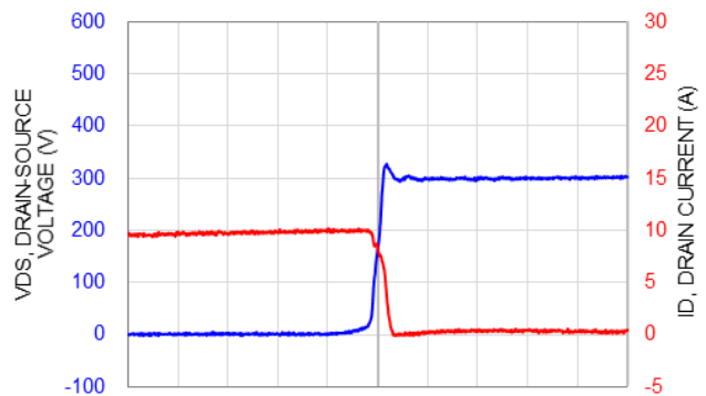
Figure 11. Turn-off Waveform T_J = 100^\circ\text{C} , V_{PN} = 300\text{ V}
