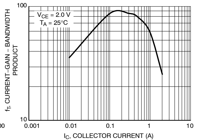
Figure 6. Current-Gain-Bandwidth Product
