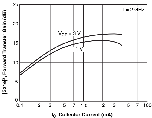
Figure 5. |S_{21e}|^2 - I_C
