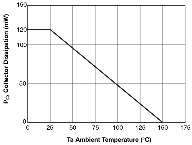
Figure 9. P_C – T_a
