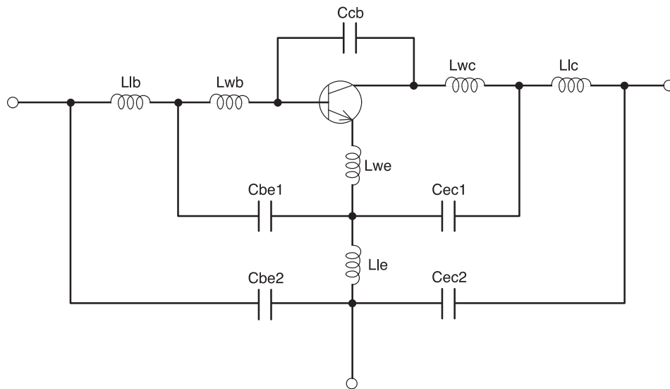
Figure 10. Schematic
