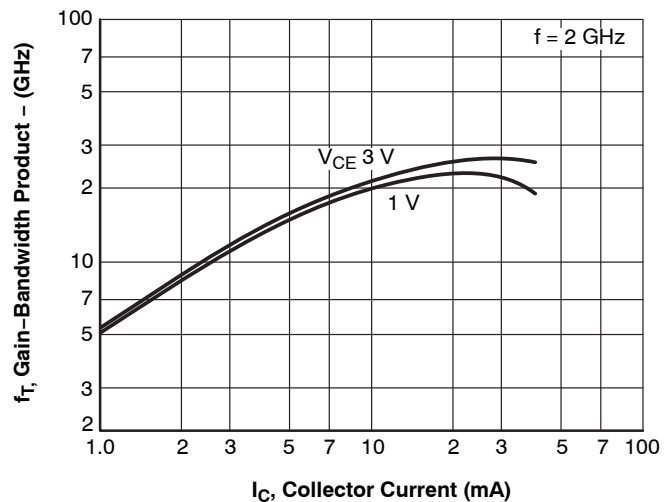
Figure 6. f_T - I_C
