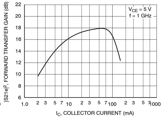
Figure 6. |S_{21e}|^2 - I_C
