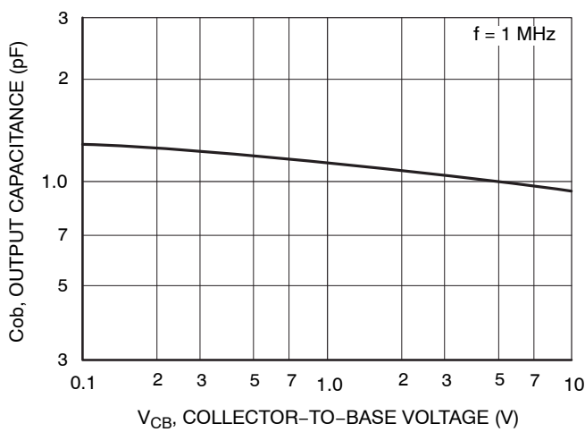
Figure 5. |C_{ob}| - V_{CB}
