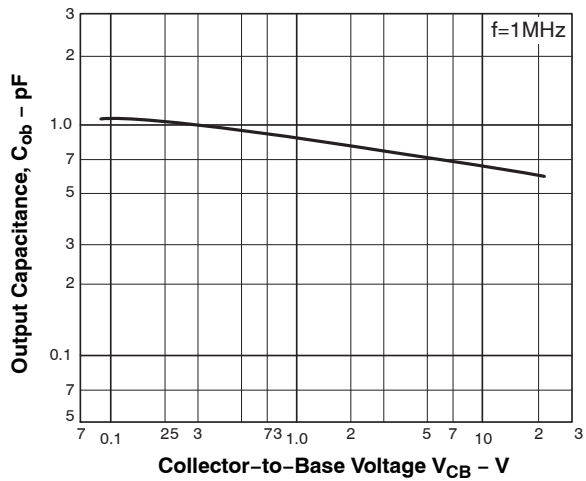
Figure 3. C_{ob} - V_{CB}
