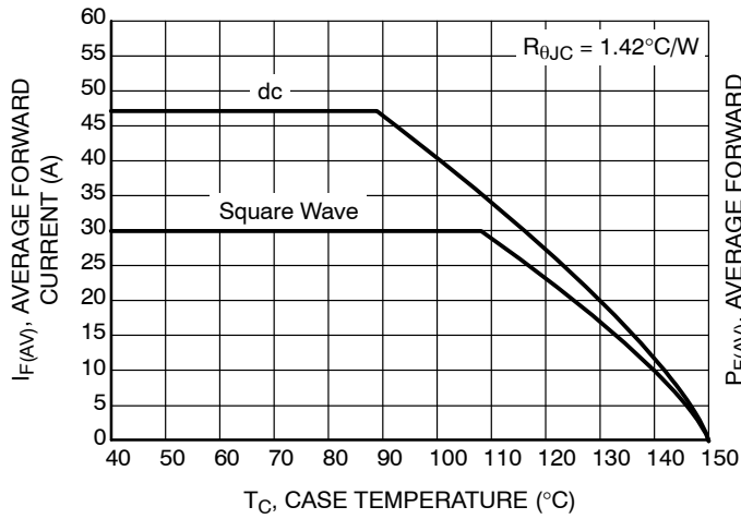
Figure 7. Current Derating per Leg
