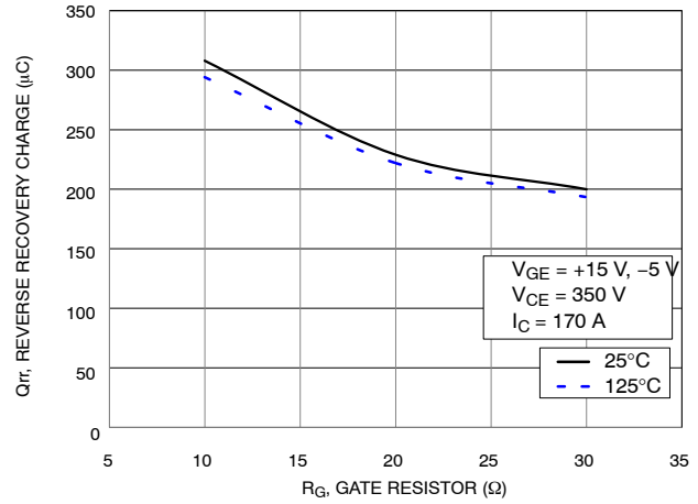
Figure 21. Typical Reverse Recovery Charge vs. R_G
