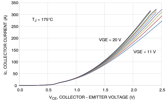
Figure 3. Typical Output Characteristics
