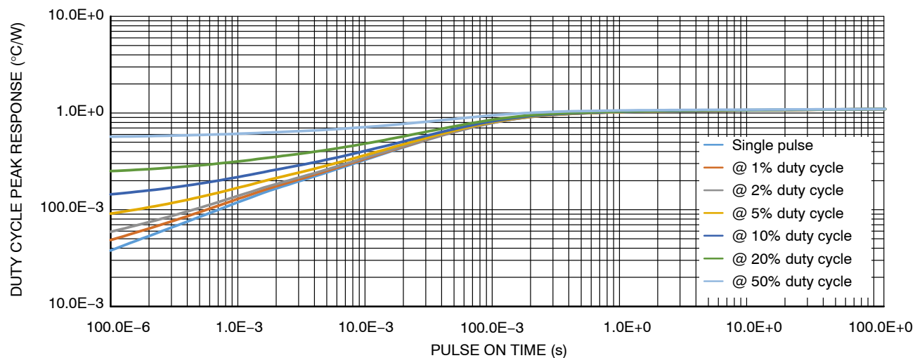
Figure 33. Transient Thermal Impedance – Diode
