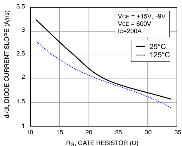
Figure 94. Typical di/dt vs. R_G
