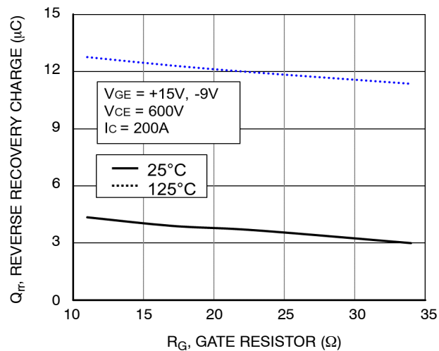
Figure 92. Typical Reverse Recovery Charge vs. R_G
