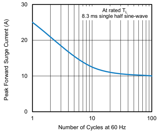
Fig. 7 - Maximum Non-Repetitive Peak Forward Surge Current Number of Cycles
