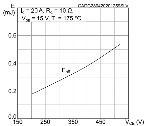
Figure 15. Switching energy vs collector emitter voltage
