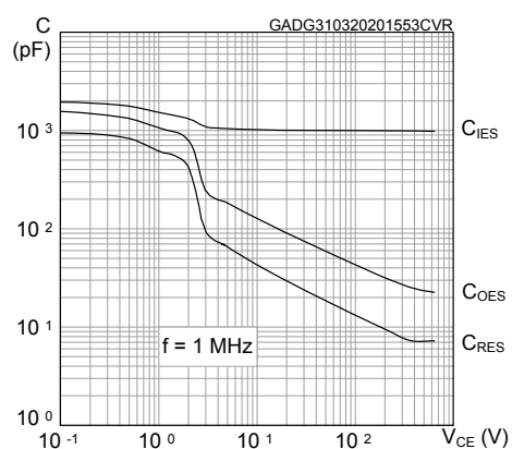
Figure 11. Capacitance variations
