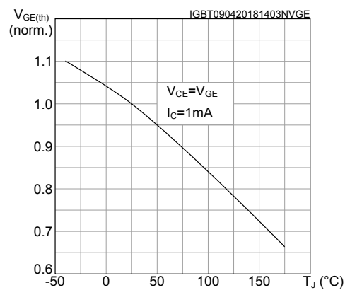
Figure 9. Normalized V_{GE(th)} vs junction temperature
