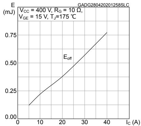
Figure 13. Switching energy vs collector current
