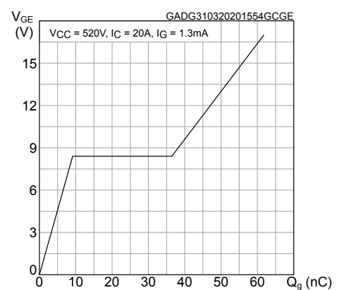
Figure 12. Gate charge vs gate-emitter voltage
