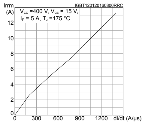
Figure 19. Reverse recovery current vs diode current slope
