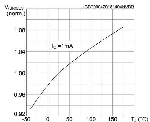
Figure 10. Normalized V_{(BR)CES} vs junction temperature
