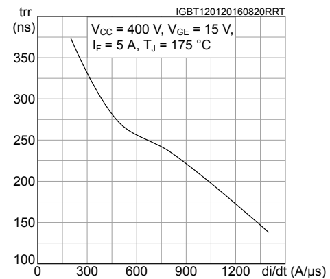
Figure 20. Reverse recovery time vs diode current slope
