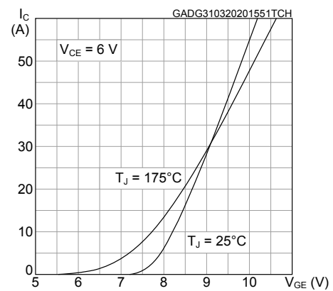
Figure 8. Transfer characteristics
