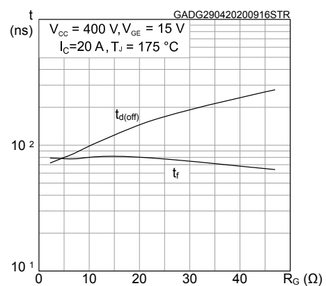
Figure 18. Switching times vs gate resistance
