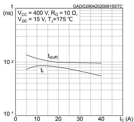
Figure 17. Switching times vs collector current
