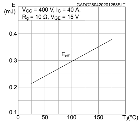
Figure 14. Switching energy vs temperature
