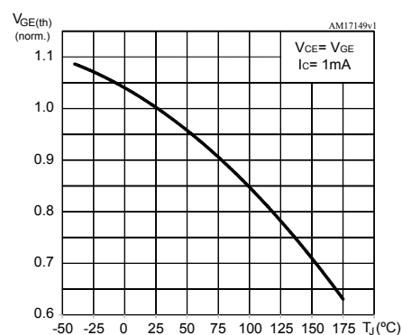
Figure 11. Normalized VGE(th) vs junction temperature
