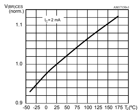
Figure 12. Normalized V(BR)CES vs junction temperature
