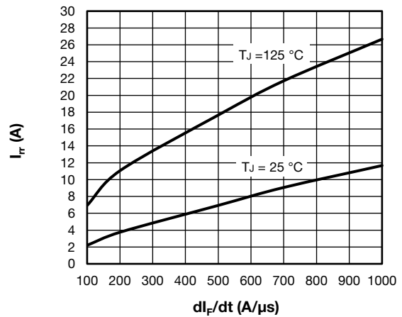
Fig. 15 - Typical Diode Reverse Recovery Current vs. dl_F/dt I_F = 50 A, V_{CC} = 200 V
