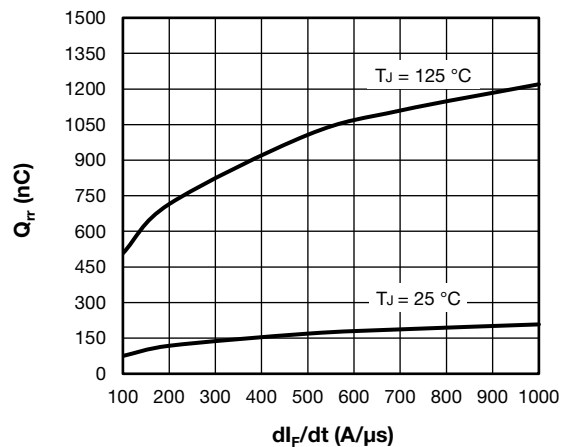
Fig. 16 - Typical Diode Reverse Recovery Charge vs. dl_F/dt I_F = 50 A, V_{CC} = 200 V
