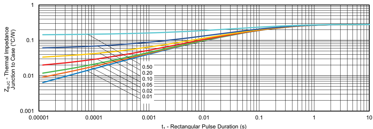
Fig. 7 - Maximum Thermal Impedance Z_{thJC} Characteristics
