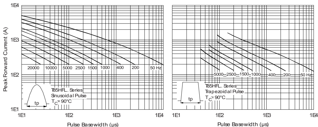
Fig. 44 - Frequency Characteristics
