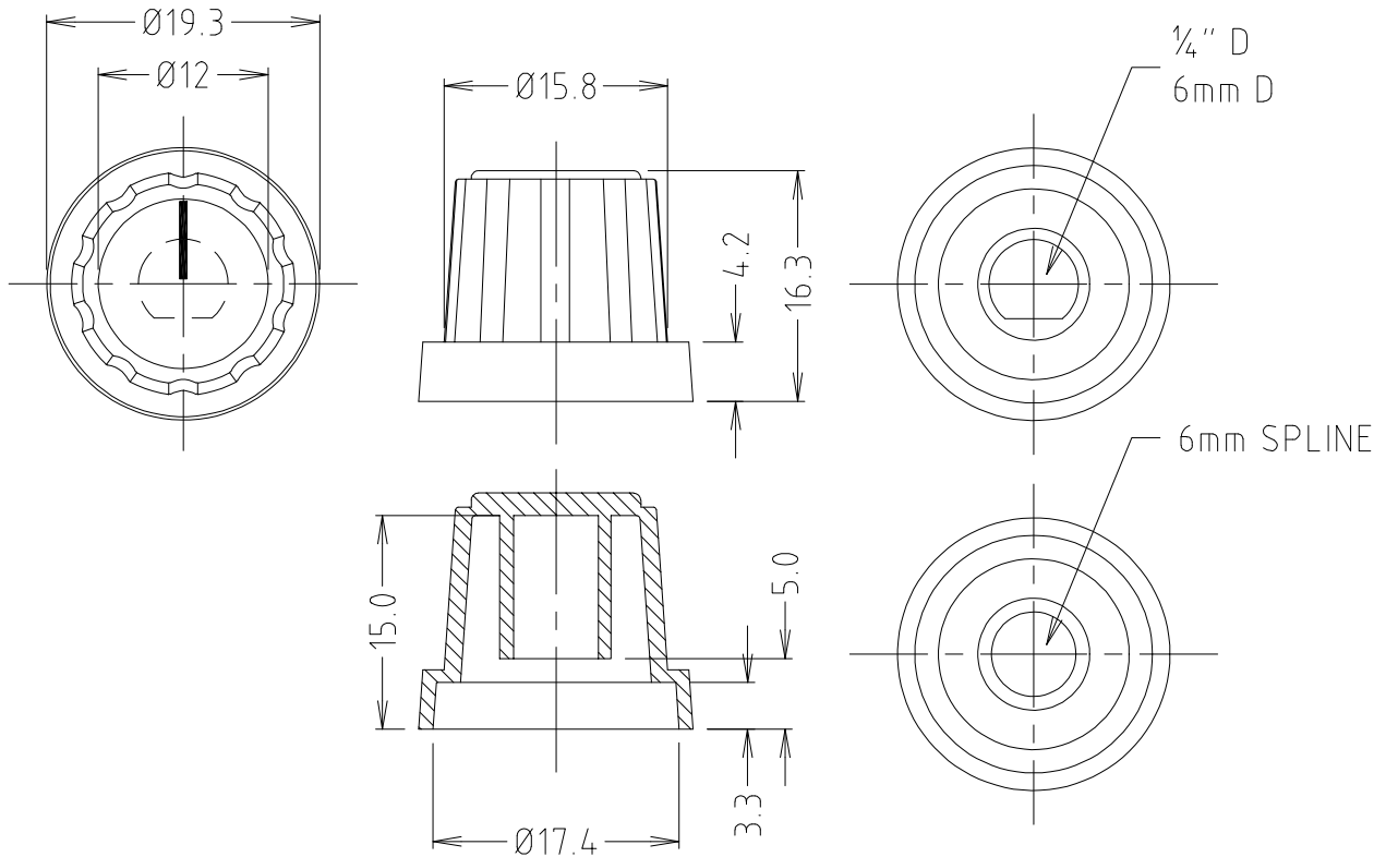
CP3450 - C18 KNOB \frac{1}{4}" D SHAFT WITH MARKER LINE CP34505 - C18 KNOB 6mm D SHAFT WITH MARKER LINE
