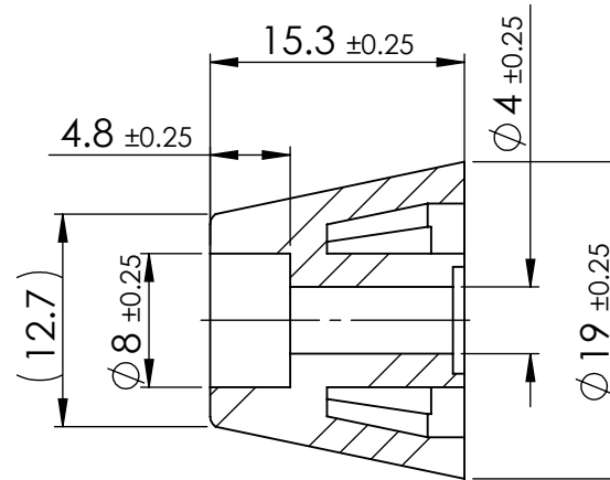
SECTION Y-Y
