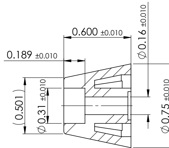
SECTION Y-Y
