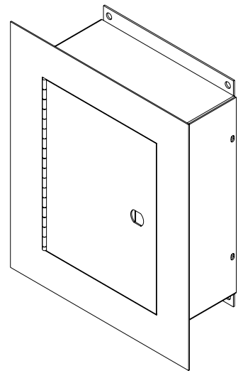
ISOMETRIC VIEW
