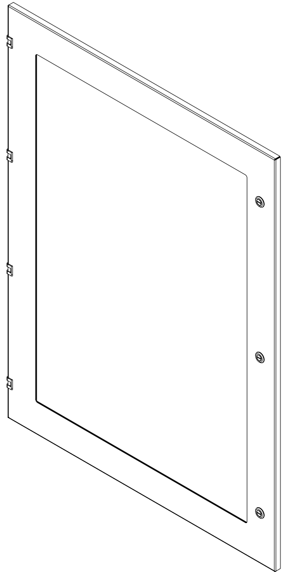
ISOMETRIC VIEW
